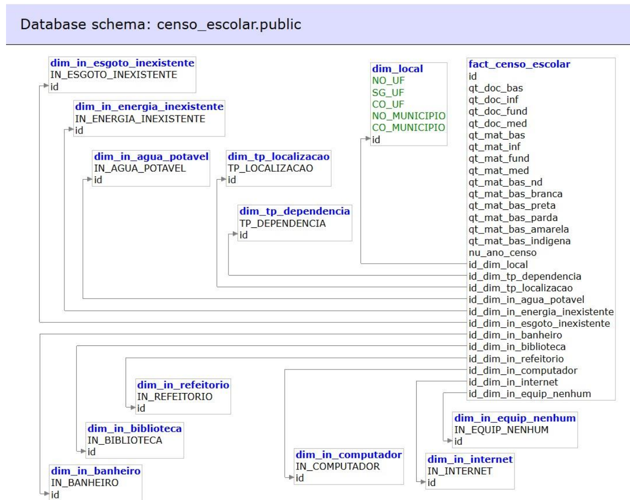
Figure 4.1 Star Schema
